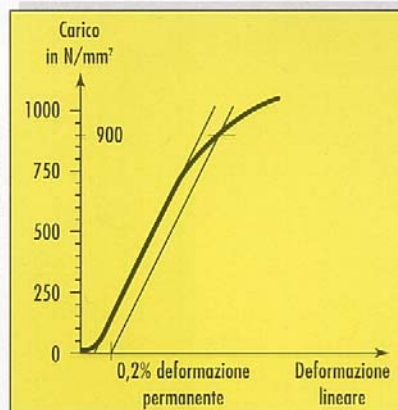
BUMAX 109:1000/900 N/mm 2
