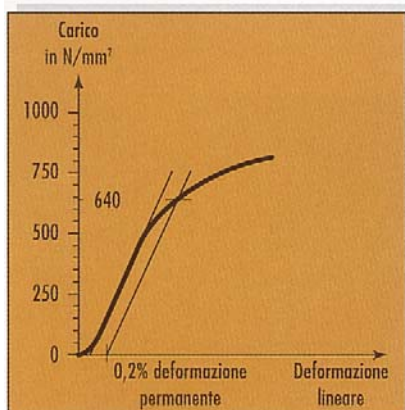
BUMAX 88:800/640 N/mm 2
